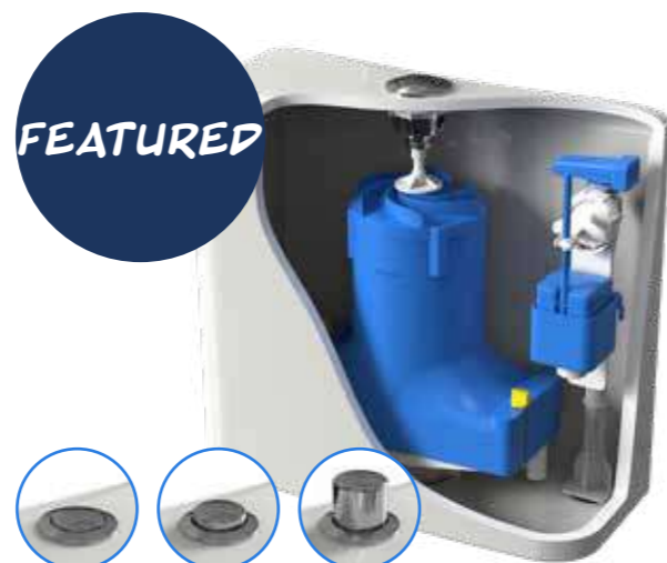
FEATURED Push button operation with a choice of caps; flush, low profile and palm push
